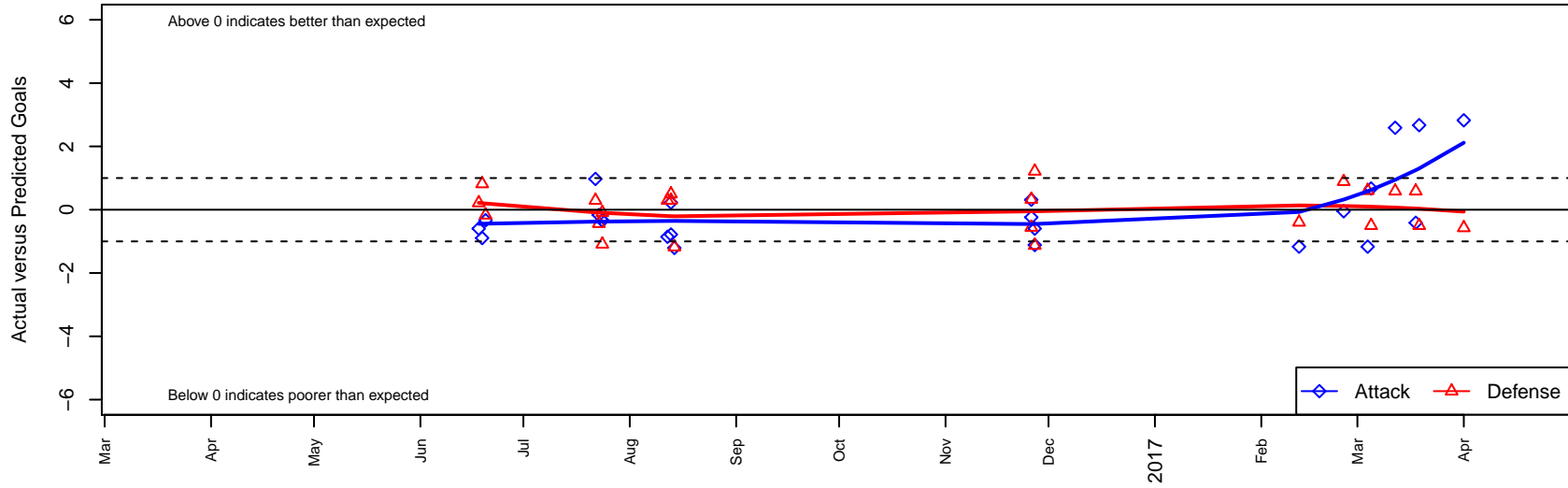
Cheney Storm FC G00 Dots are actual minus expected GF (blue circles) and GA (red triangles). Blue line is smoothed change in attack strength. Red is smoothed change in defense strength.
